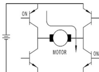
Forward run - upper left and lower right transistors on
