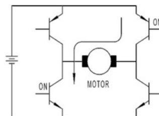
Reverse run - lower left and upper right transistors on
