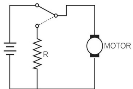
Maximum braking effect is obtained when R = 0
