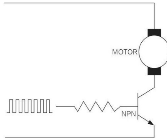
PWM control reference circuit diagram
