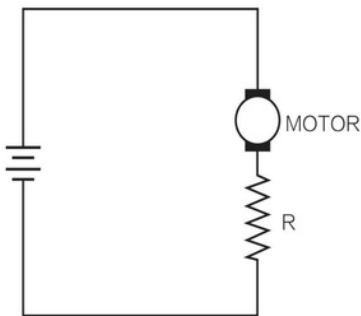
Series resistance controls the motor current and speed
